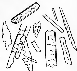
Fig. 19.—BENZOIC ACID.
